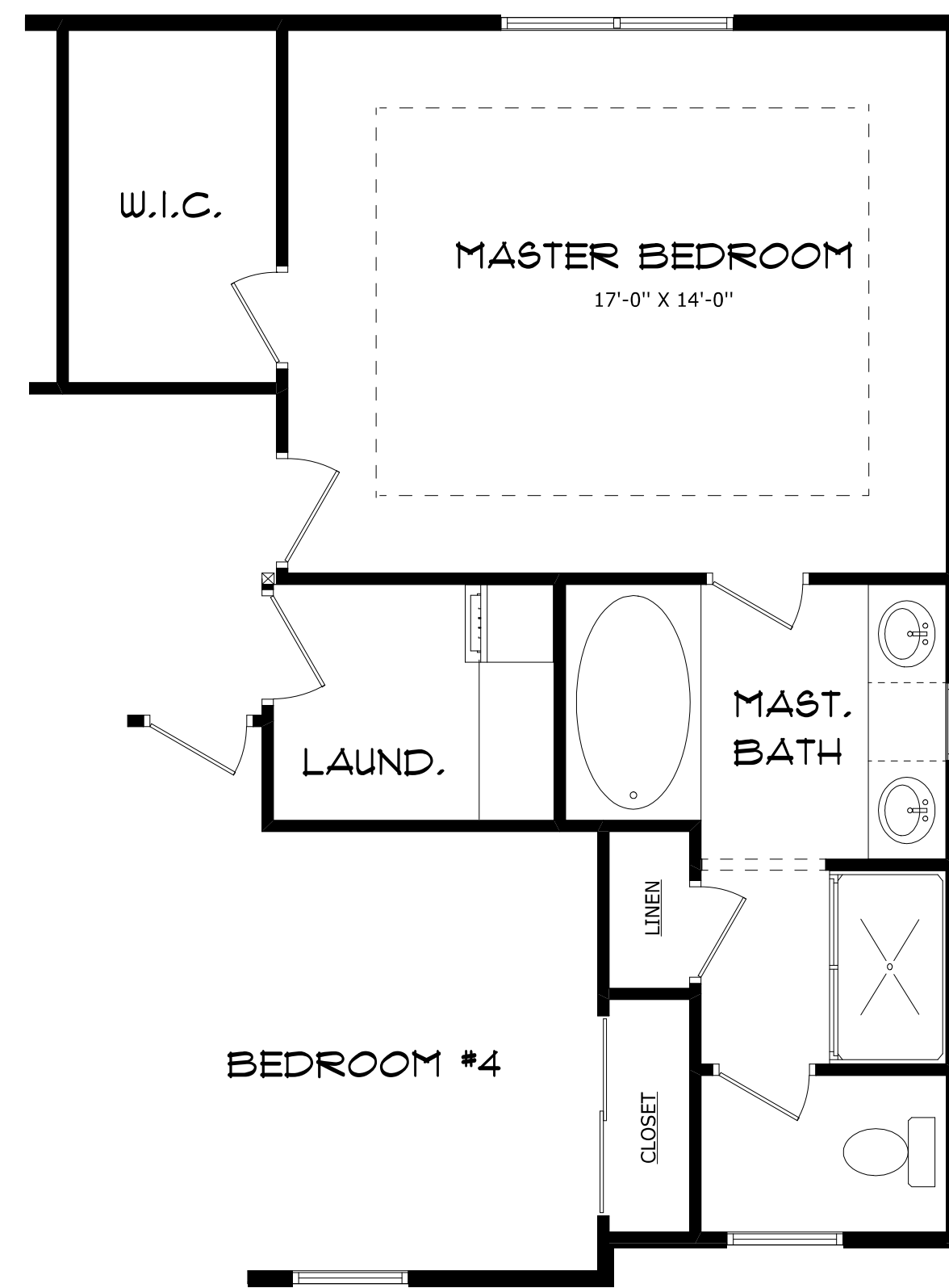
OPT. SECOND FLOOR PLAN
