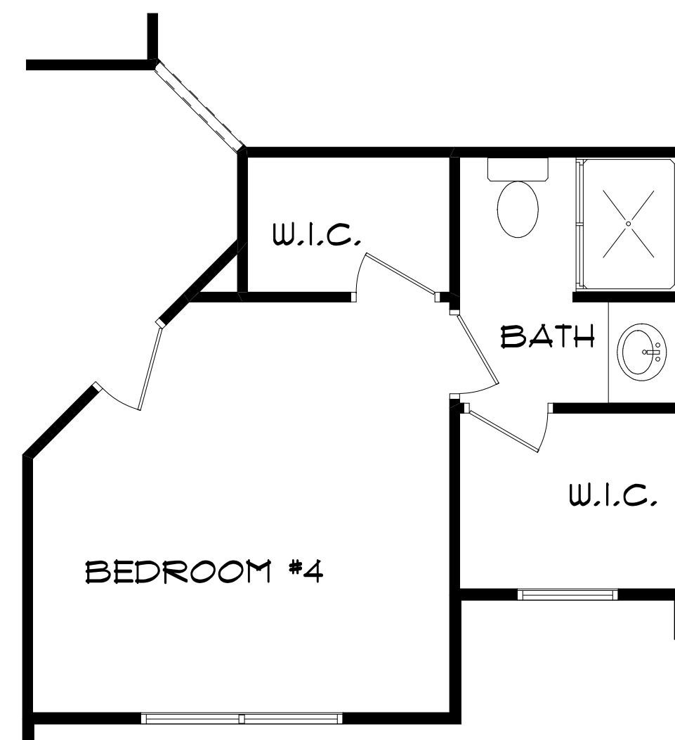
ALT. SECOND FLOOR PLAN
